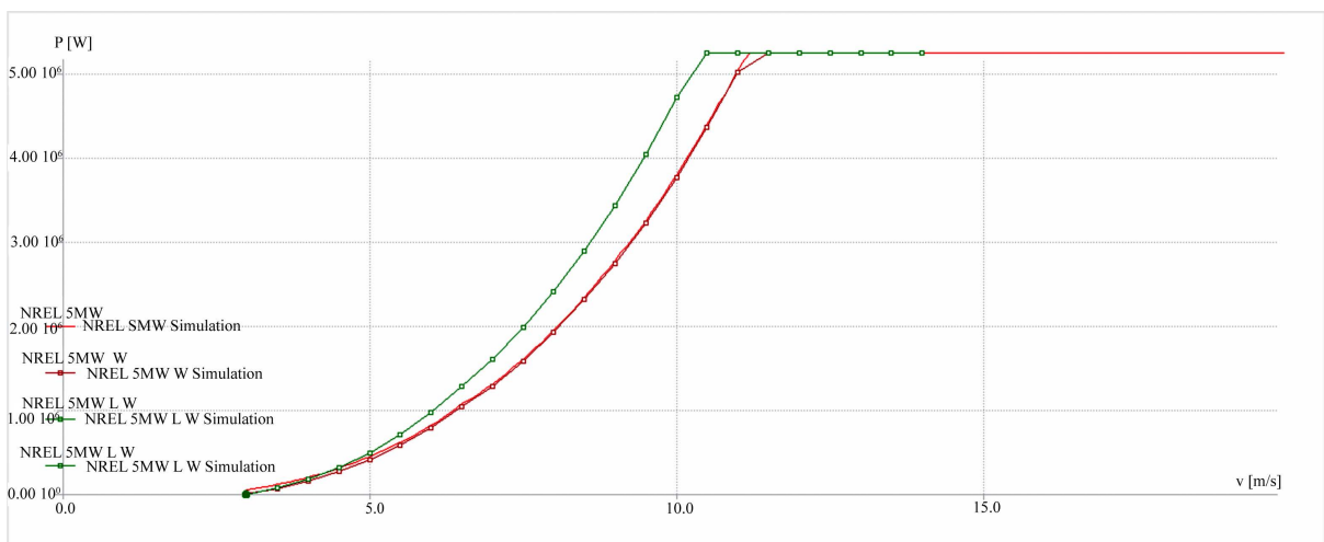
Figure 4. Summarizes change in power output for variation in chord of the blade proportion to the radius and also for varying the chord alone.
