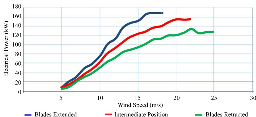
Figure 5. Reproduced experimental, proof-of-concept power curve for variable length wind turbine by Mark H. Dawson et al. [17].
