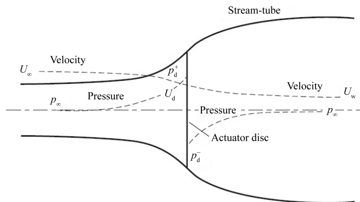
Figure 2. An energy extracting actuator disc and stream tube.
