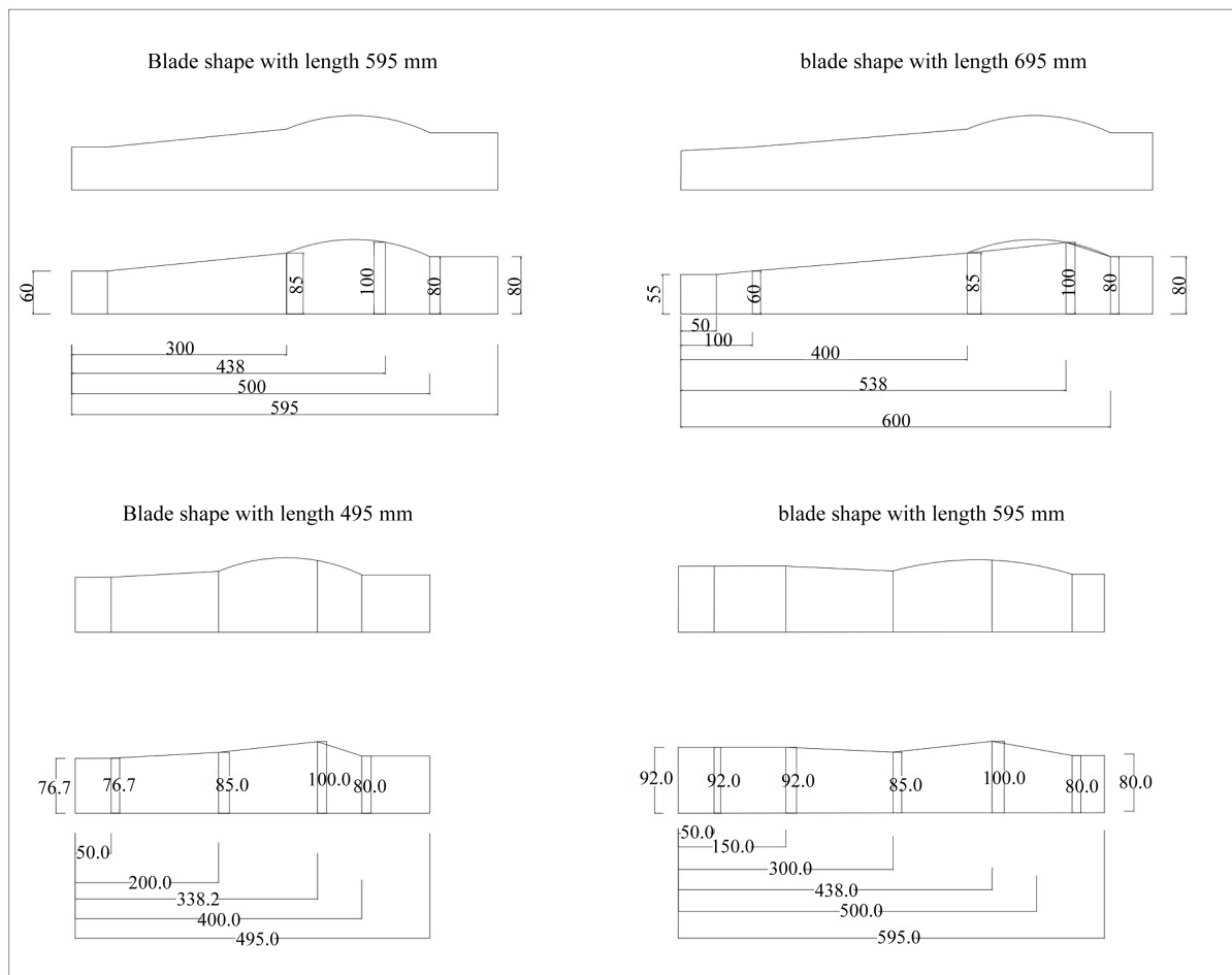
Figure 1. Blade profile diagrams.
