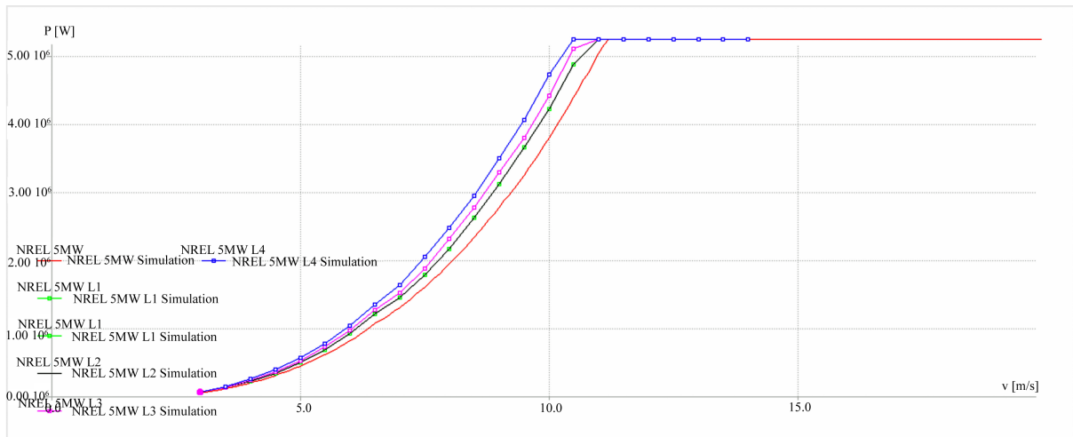
Figure 3. Graphical summary of simulation for variation in radius.
