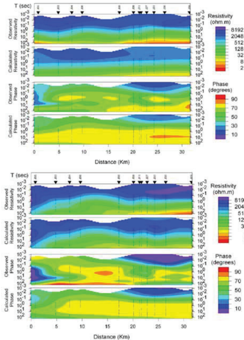
Figure 6. Pseudo sections of apparent resistivity and phase for the derived 2-D model in both TE and TM mode.
