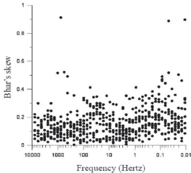
Figure 3. Dimensionality parameter-skew with < 0.3 for many frequencies indicating that the impedance data belong to 2-D rather than 3-D. Some data points > 0.3 reflect the 3-D nature due to near surface inhomogeneities.
