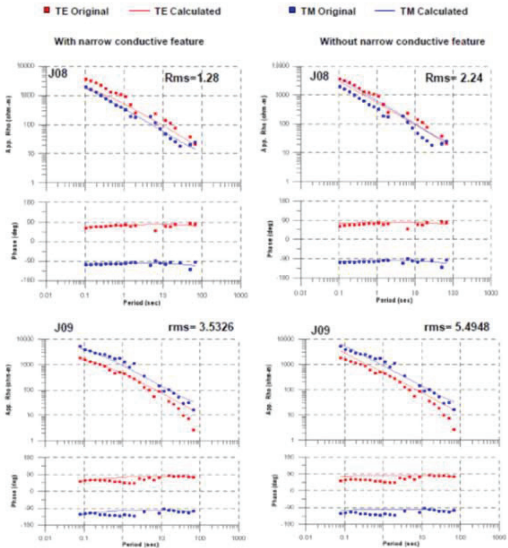
Figure 7. The forward response with and without less resistive narrow feature for the station J08 and J09.
